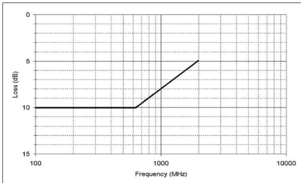
Figure 33-8. Minimum Differential Output Return Loss
